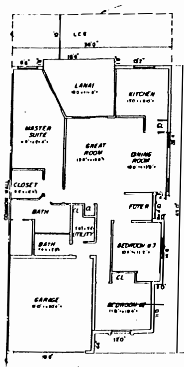
ASHLEY III SCALE 1/8" = 1'-0"
